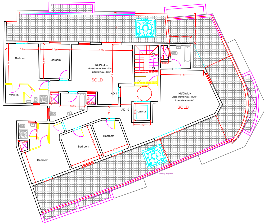
Approved/ Proposed Level 3 Scale 1:100
