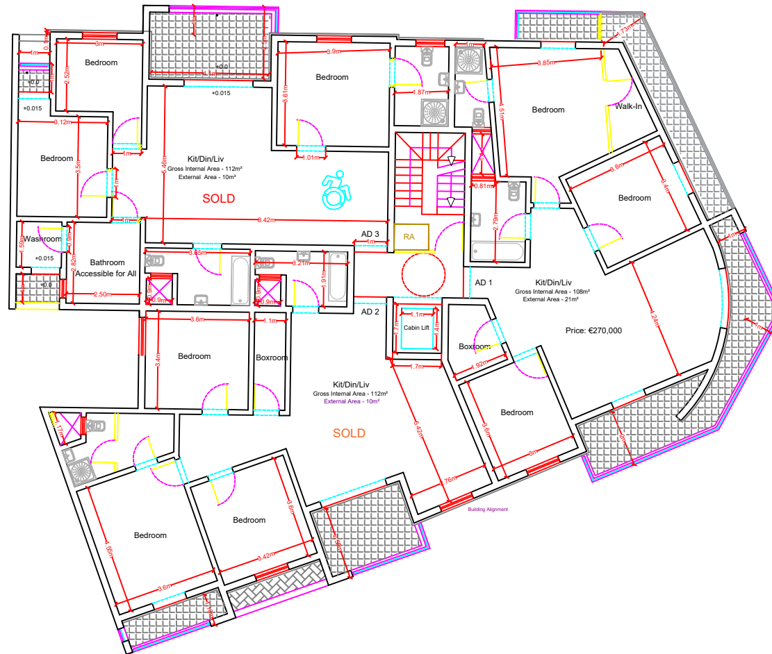
Approved/ Proposed Level 0 Scale 1:100
